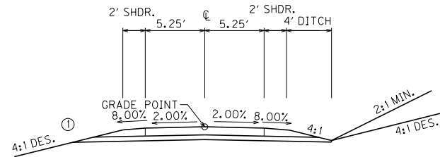
NORMAL SECTION CR 3035
